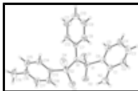
Fig. 1. The molecular structure of (I) showing the atomic numbering and 40% probability displacement ellipsoids.
